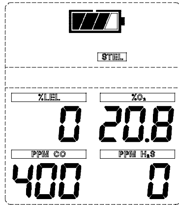
Figure 3-12. Exposure Page with STEL Alarm
