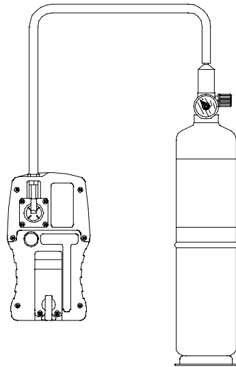
Figure 3-5. Pumped Instrument with Calibration Tubing
