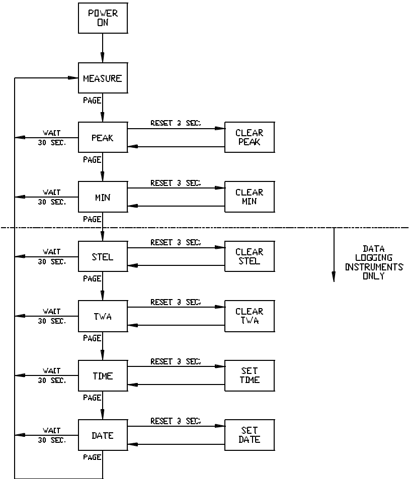
Figure 3-9. Flow Diagram
