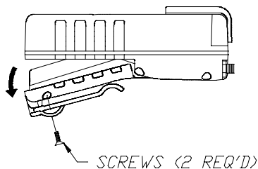
Figure 4-1. Removing the Battery
