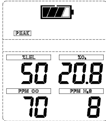
Figure 3-10. PEAK Readings on the Display
