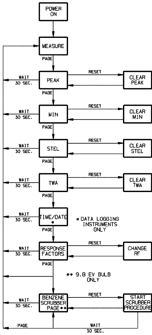
Figure 3-9. Flow Diagram
