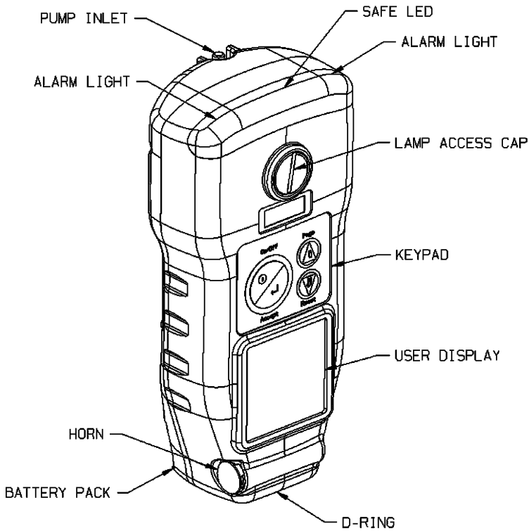
Figure 3-1. Instrument Features
