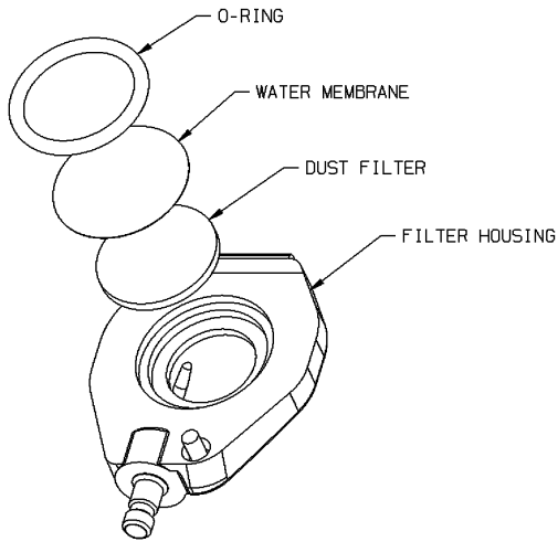
Figure 6-5. Filter Installation
