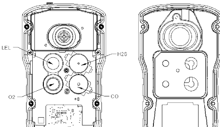
Figure 6-8. Sensor Locations
