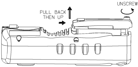
Figure 4-1. Battery Pack Removal
