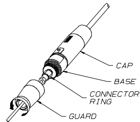
Figure 2-23. Attaching Probe to Sample Line
