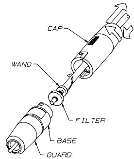
Figure 2-24. Changing the Probe Filter
