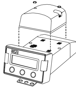
Figure 2-22. Pump Installation
