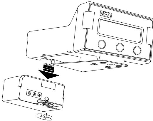
Figure 2-1. Battery Pack Installation
