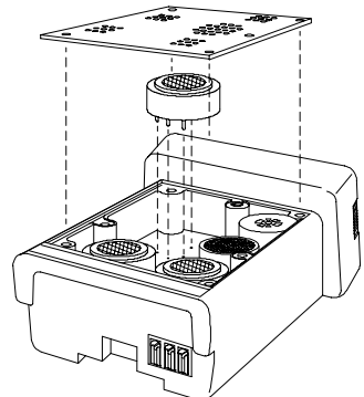
Figure 3-1. Sensor Cover Plate
