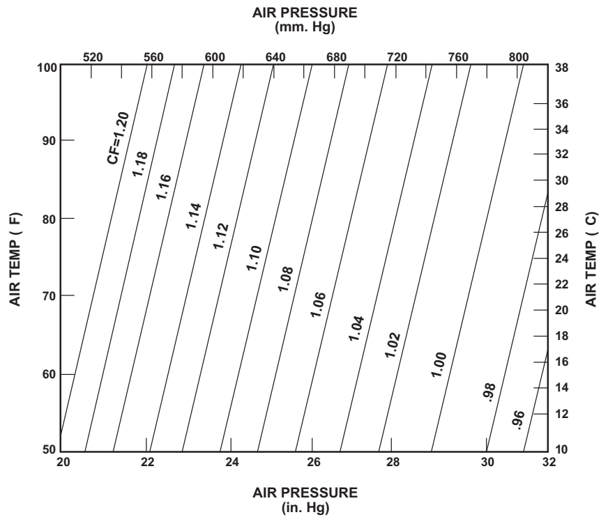
Velometer correction factors
